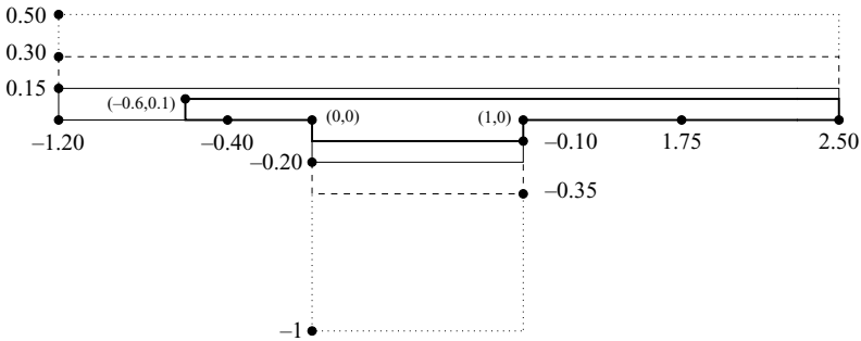
FIGURE 7. Mesh structure for the open cavity flow. The thick solid line is characterized by the vertex density n . The thin solid line, dashed line and dotted line appearing in the upper part of the mesh, i.e. in the open flow, are, respectively, characterized by the vertex densities n_1^+ , n_2^+ and n_3^+ . The same lines in the lower part of the mesh, i.e. in the cavity region, are, respectively, characterized by the vertex densities n_1^- , n_2^- and n_3^- .
